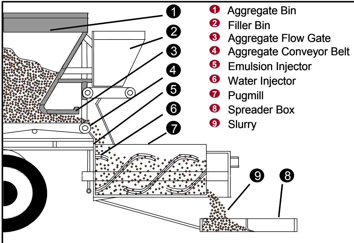
Figure 2- Cross Section of truck
