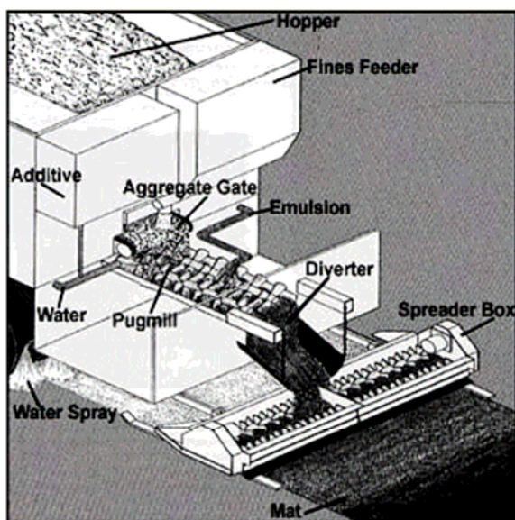
Figure 1- Schematic of a Slurry Surfacing Machine
