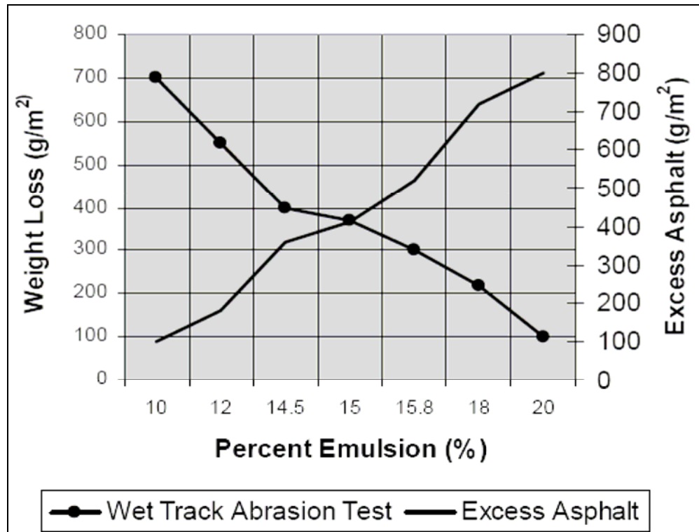
Figure 7- : Determining Optimum Binder Content
