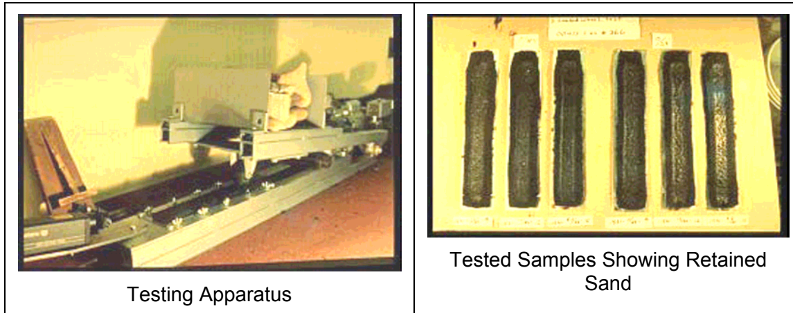
Figure 6- Loaded Wheel Test and Excess Asphalt Test Apparatus and Test Samples
