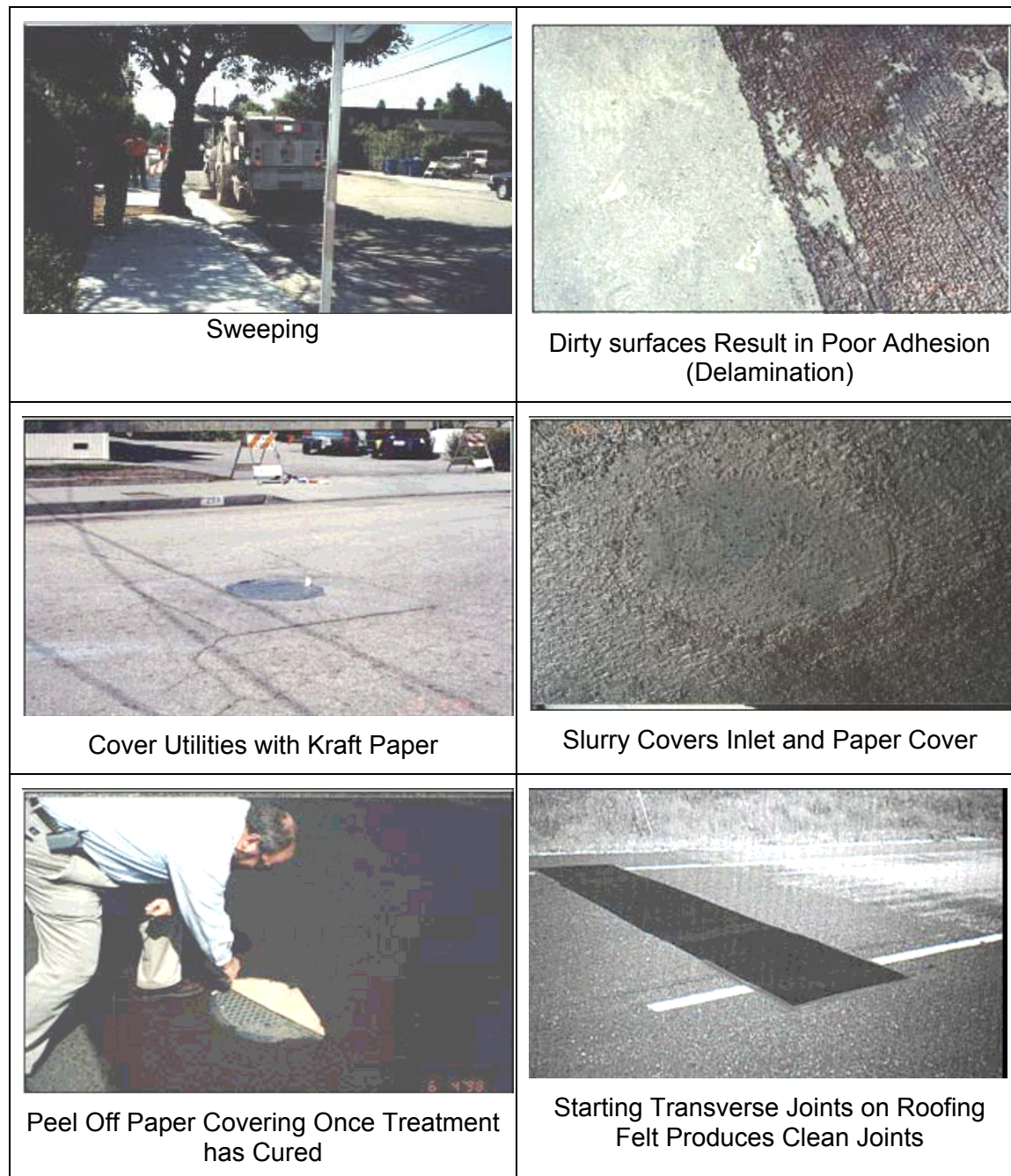
Figure 11- Surface Preparation Methods
