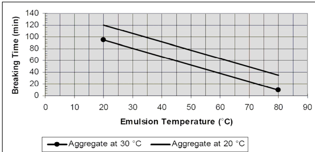
Figure 12- Effect of Temperature on Break Rate
